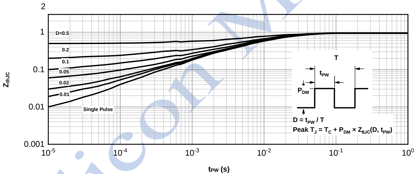
Fig.15 Transient thermal impedance from junction to case
