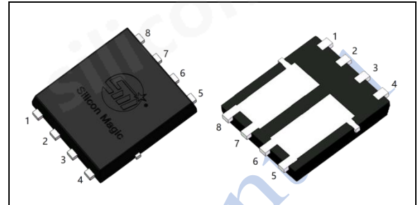
PDFN5*6-D_A3
