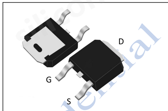
TO252-3L
